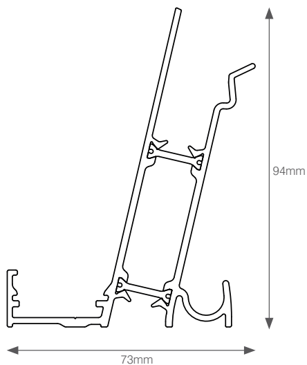
EAVES BEAM A-05004
