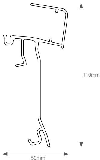
GLASS RETAINER A-05077
