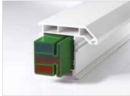
PVC-U thermal inserts in the frame
